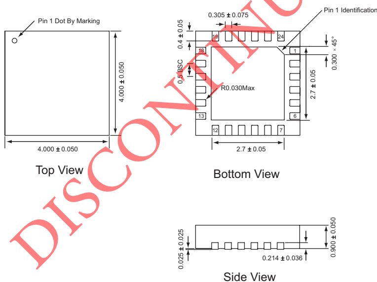
QFN44-24 3
