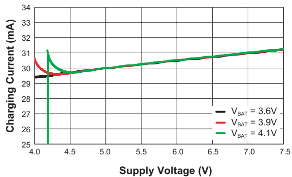
Constant Charging Current vs. Supply Voltage ( I_{CH} = 30mA )
